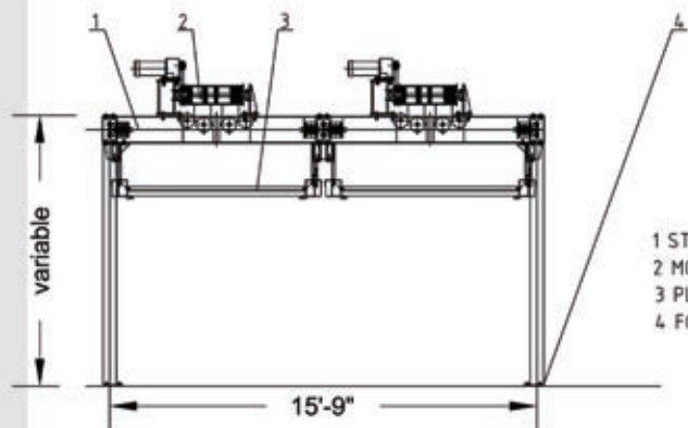
SP100 FRONT/REAR ELEVATION
