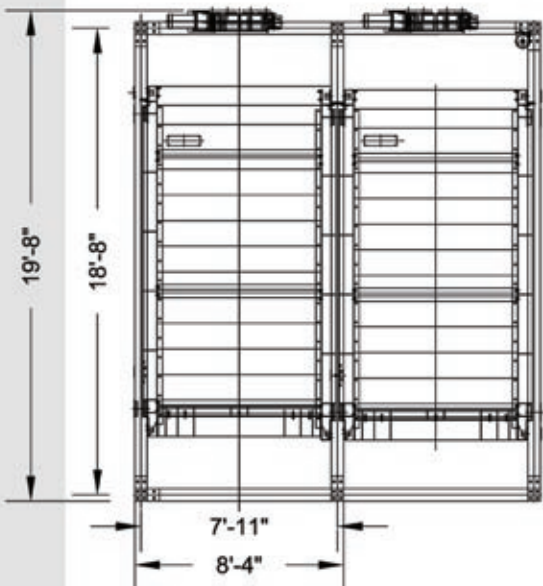
SP100 SCHEMATIC PLAN
