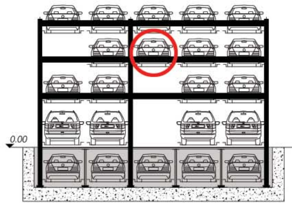
2. Slide-motion initiated.
